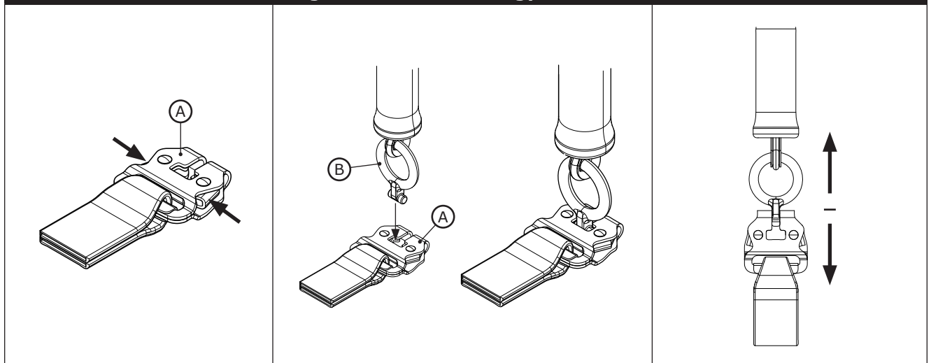
Figure 9 - Modular Energy Absorbers
