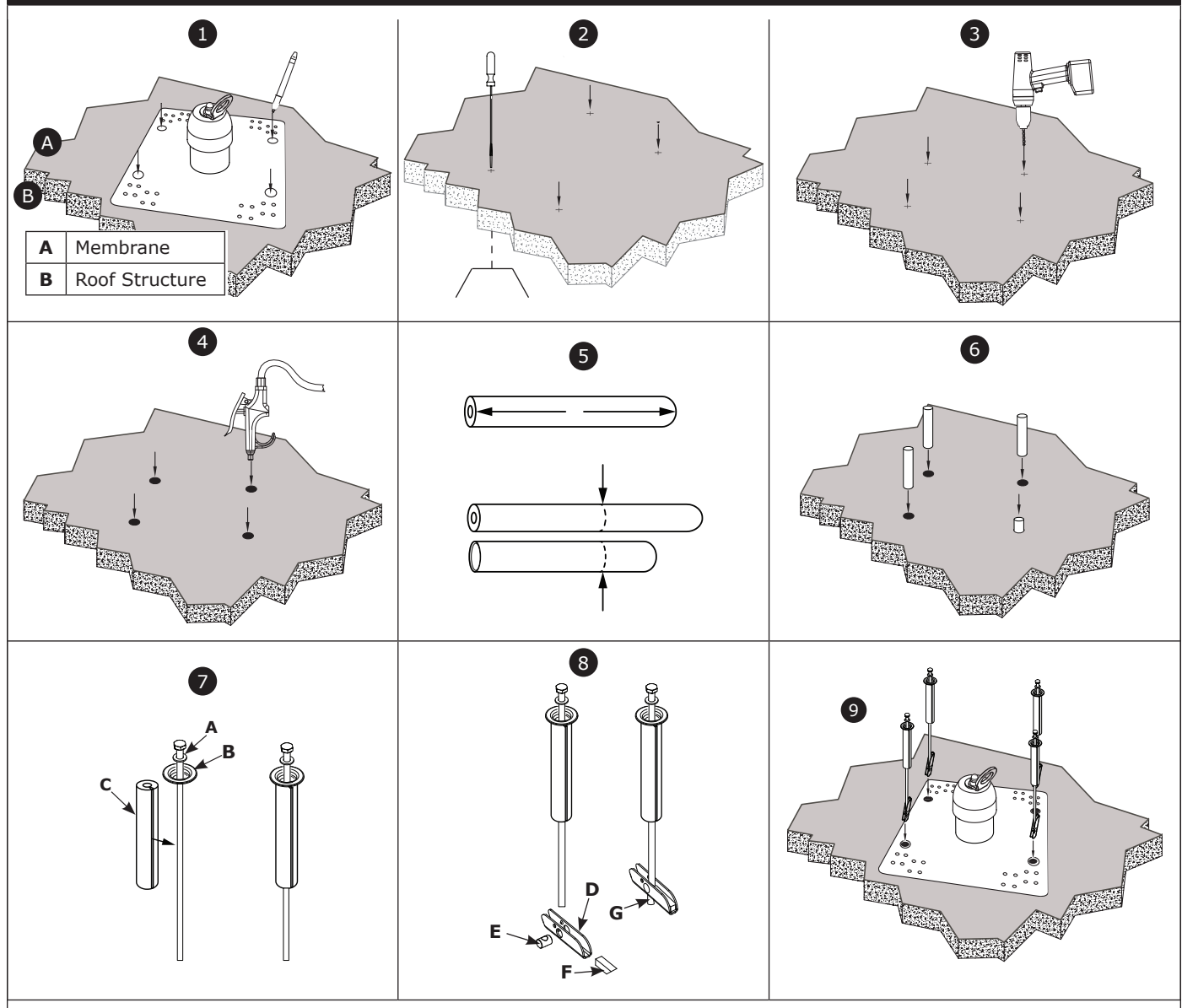
Figure 10 – Installation Using Toggle Bolts
