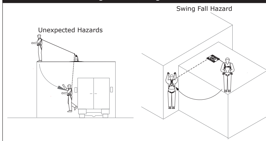
Figure 2 – Swing Falls
