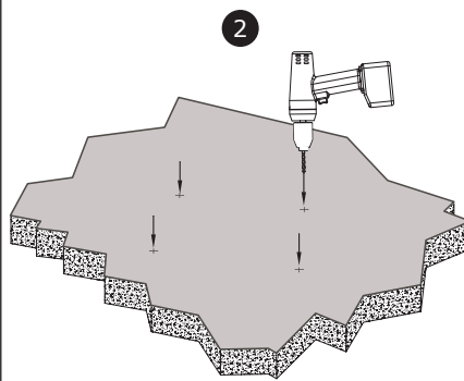
Figure 9 – Installation on Concrete Roof Decks
