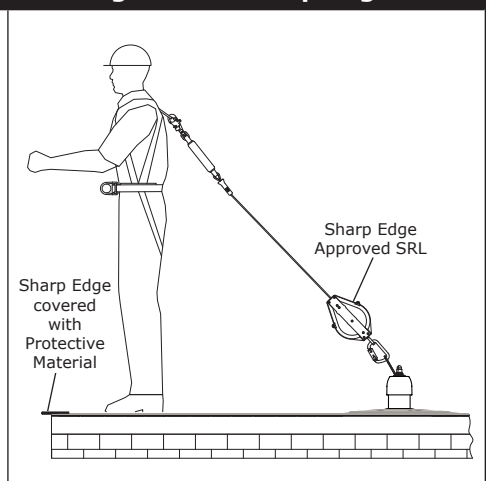
Figure 3 – Sharp Edges
